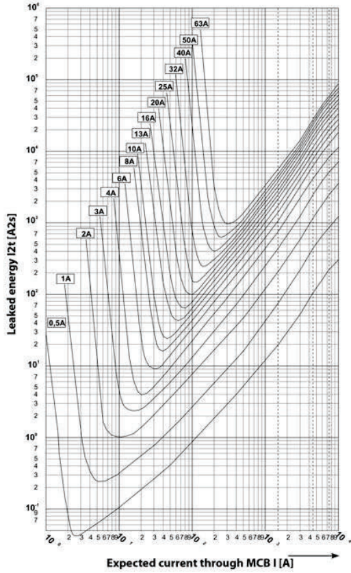
Charts of leaked energy I^2t of MCBS PR 60 with tripping characteristic B
