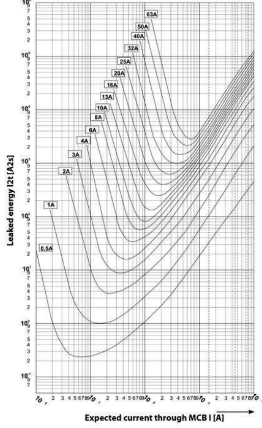
Charts of leaked energy I^2t of MCBS PR 60 with tripping characteristic C
