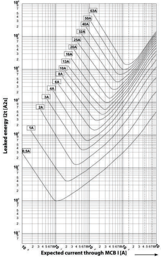
Charts of leaked energy I^2t of MCBS PR 60 with tripping characteristic D
